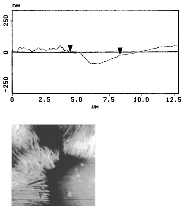
Figure 6. Height profile across the crystalline/melt interface for a growing PEO spherulite.
